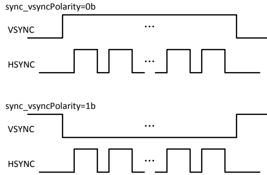
Figure 11 Vsync polarity
