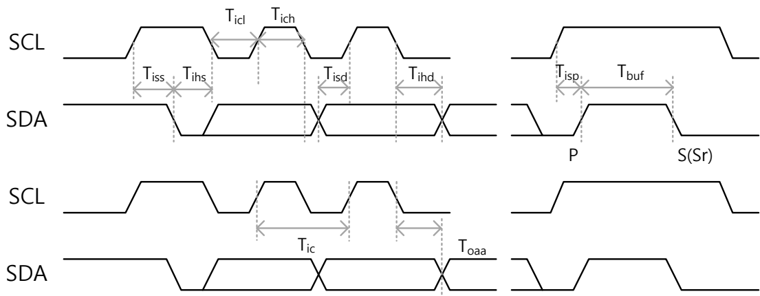
Figure 35 Timing diagram of SCL and SDA
