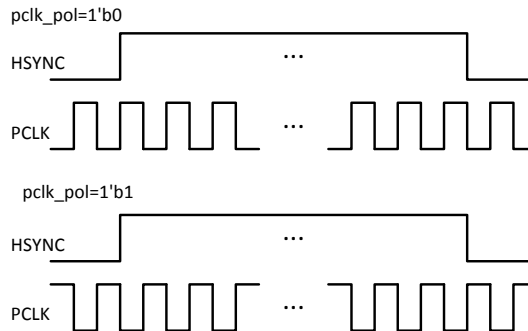
Figure 11 PCLK polarity
